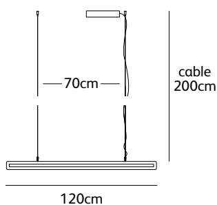
FR.120.SU.UP/DOWN.*
